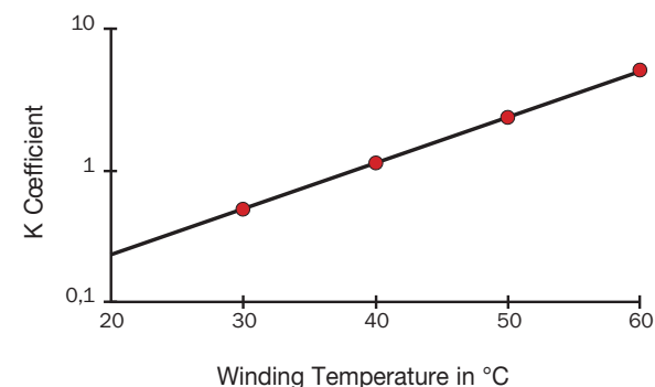
Correction of insulation resistance according to temperature (source IEEE - 43-2000)
